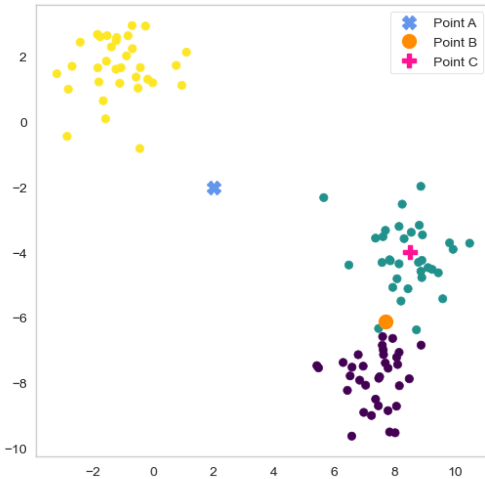
Fig. 1: Depending on the where the hiker is standing he makes the the conclusion that is either in a birch or spruce forest.
