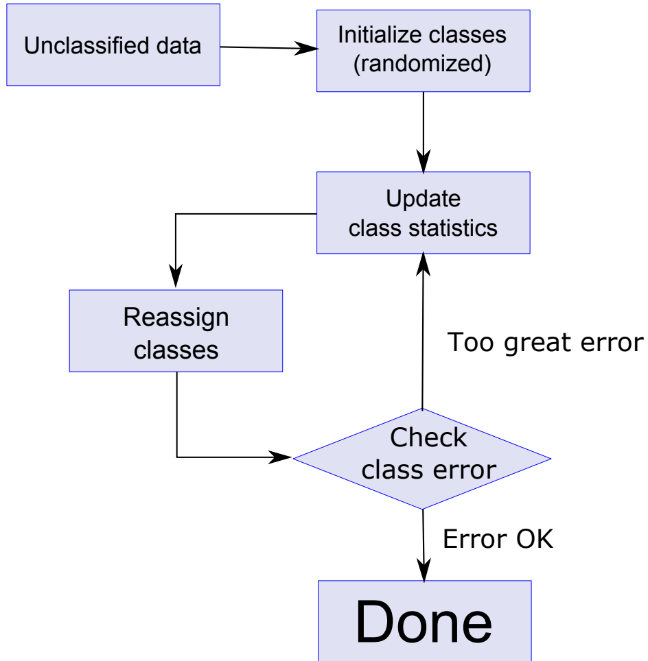
Fig. 1: Flow chart for the k-means clustering iterations.
