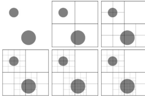
Fig. 1: A quad tree decomposition.
