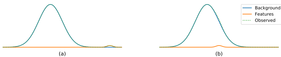
Fig. 3: Two cases of unbalanced data; (a) the classes are well separated and the feature class is clearly visible in the tail distribution of the background and (b) the feature class is embedded in the background making it hard to detect.
