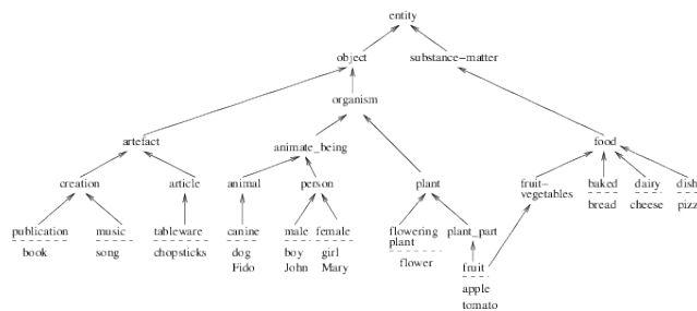
Fig. 2: Hierarchical structure of the WordNet database.
