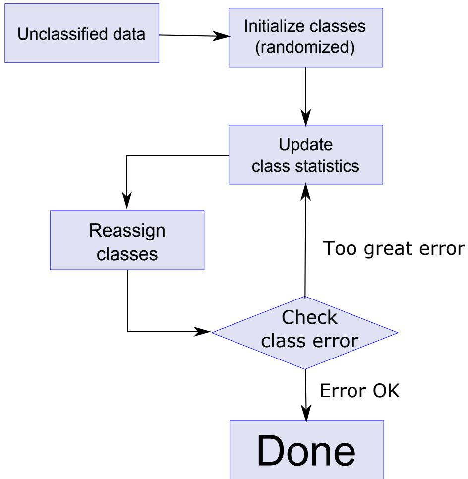
Fig. 7.1: Flow chart for the k-means clustering iterations.
