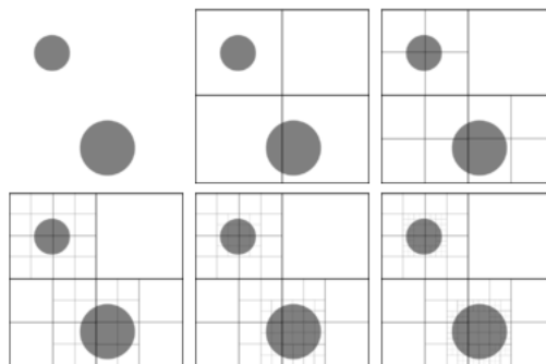
Fig. 8.1: A quad tree decomposition.
