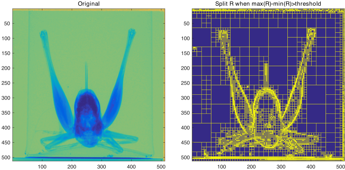
Fig. 8.2: A neutron radiograph of a grasshopper decomposed using a quad tree.
