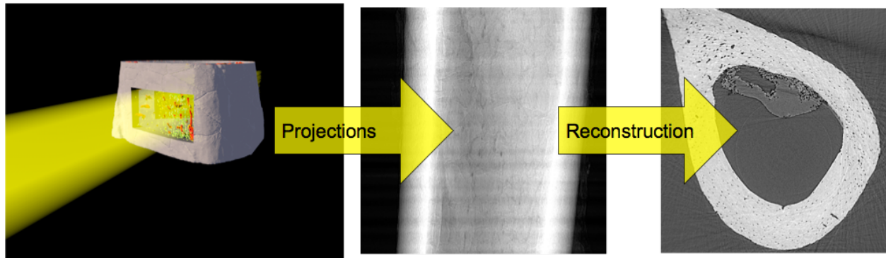
Fig. 5.1: Acquisition workflow to obtain CT slices of a specimen.
