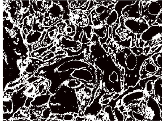
True Positive (13681)
