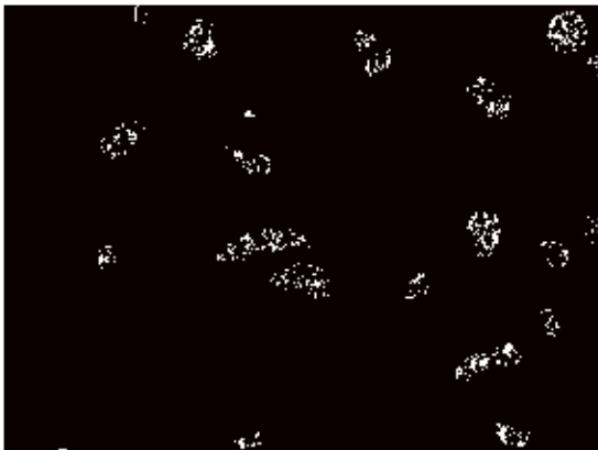
False Negative (2932)
