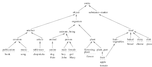
Fig. 5.2: Hierarchical structure of the WordNet database.
