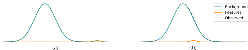
Fig. 8.3: Two cases of unbalanced data; (a) the classes are well separated and the feature class is clearly visible in the tail distribution of the background and (b) the feature class is embedded in the background making it hard to detect.
